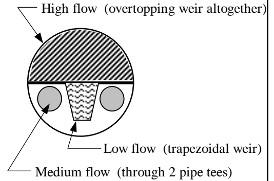
Closeup of Section A-A (flow control)
