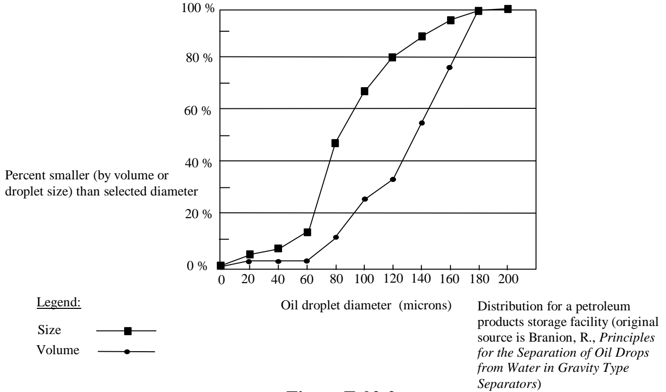
Figure F-02-2 Typical Size and Volume Distribution of Oil Droplets
