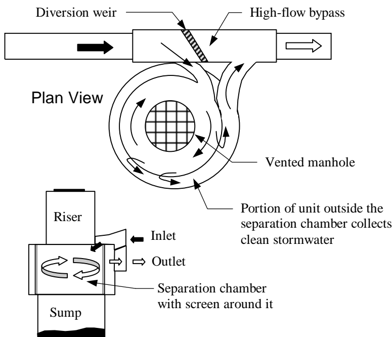
Figure F-02-6 Flow Schematic for Continuous Deflection Separators (CDS Technologies)
