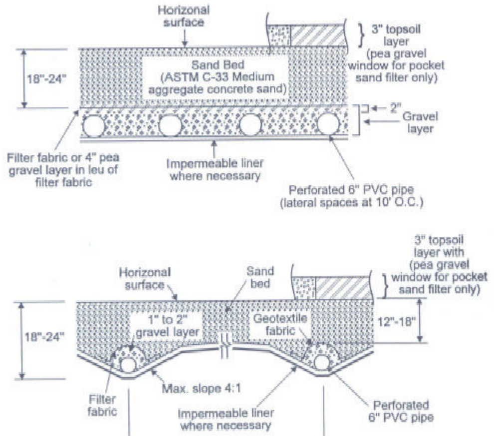
Figure F-04-2 Typical Sand Filter Media Cross Sections
