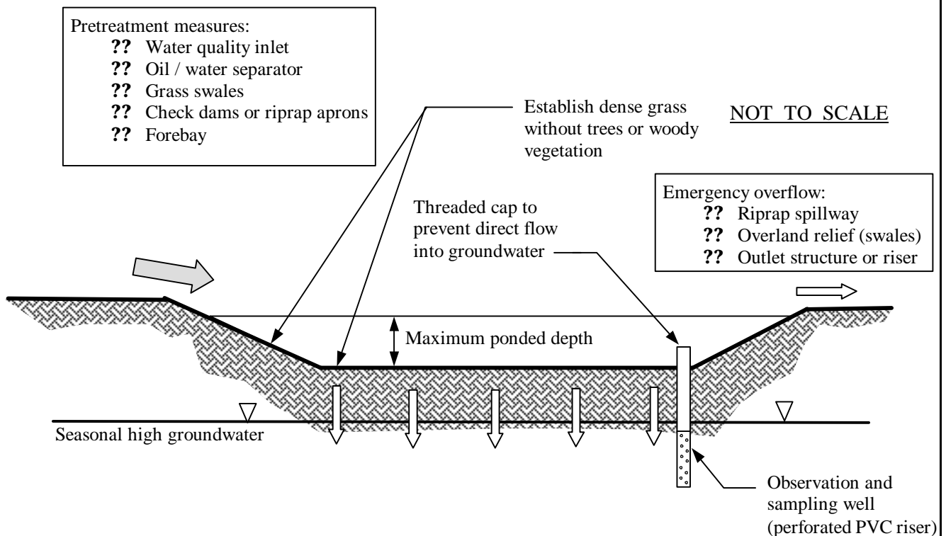
Figure I-02-2 Typical Infiltration Basin
