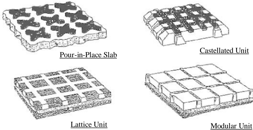
Figure I-04-2 Examples of Porous Pavement Systems
