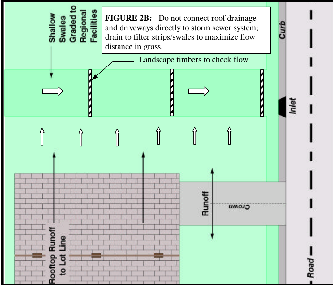
Figure O-01-2 Examples of Filter Strips and Swales
